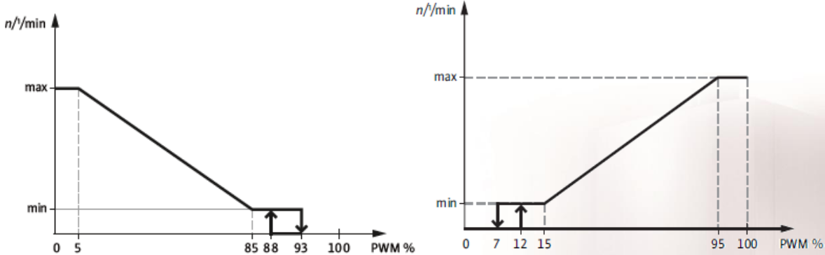
iPWM signal logic 1 (heating) (%):
